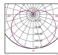
LED A60I 11W 180°
