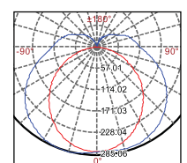
NBTLED T5D14/12 160°
