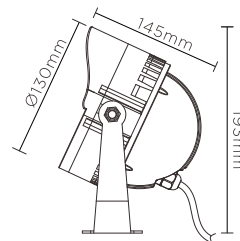
NFLED4013 Windage: 0.017m 2 Weight: 1.7kg
