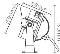
NFLED4012 Windage: 0.008m 2 Weight: 0.9kg
