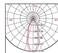
NLED1152N 50W 40°
