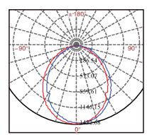
NDLLED9508P 40W 90°
