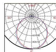
NPNLED4513 37W 110°
