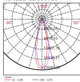
NCNLED102 80W 30°
