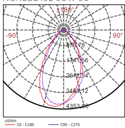
NCNLED102 60W 60°
